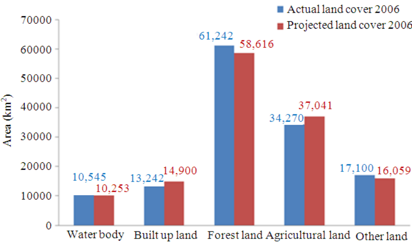
Fig. 6. Simulated versus actual LCLU classes area (km²) in 2006
